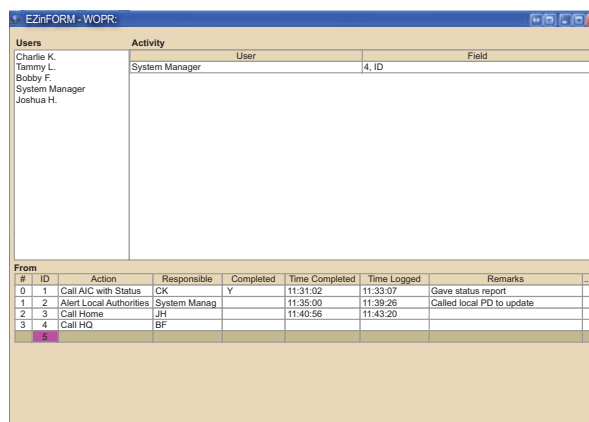
The EZinFORM editor window shows who is currently viewing the document and who is editing which cells.
